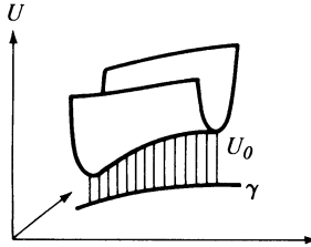
Figure 55 Potential energy U_N
