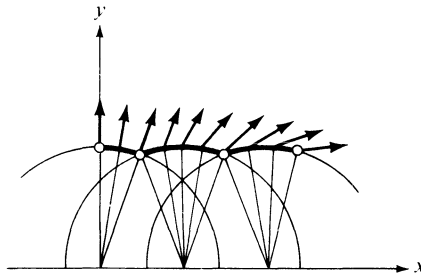
Figure 232 Parallel translation on the Lobachevsky plane
