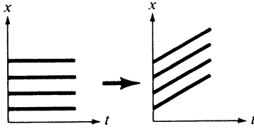
Figure 5 Galileo's principle of relativity
