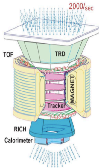
Figure 22.6. The Alpha Magnetic Spectrometer, AMS-02 (Gentile, 2003). The detector components are. Transition Radiation Detector (TRD), Time-of-flight Scintillators (TOF), Silicon Tracker (Tracker), Ring Imaging Cherenkov detector (RICH), lead/plastic fiber calorimeter (ECAL), the anticoincidence counters are located in the inner side in the magnet. The arrows represent the acceptance of CR particles, \sim 2000 \text{ s}^{-1} .
