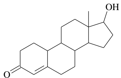
19-nor-testosterone
