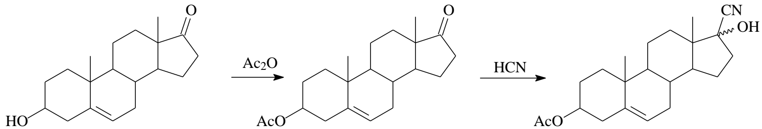
dehydroepiandrosterone
