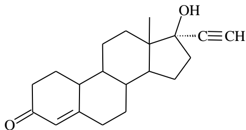
norethindrone
