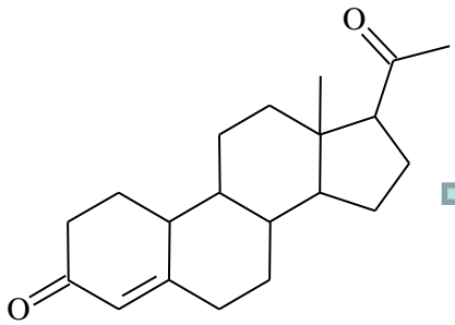
19-norprogesterone
