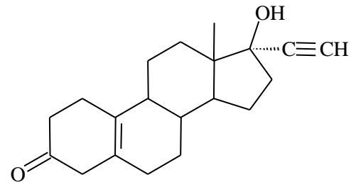
norethynodrel
