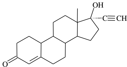
norethindrone
