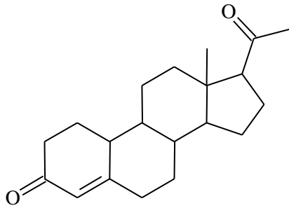
19-norprogesterone
