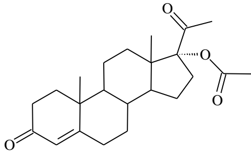
17α-hydroxyprogesterone acetate
