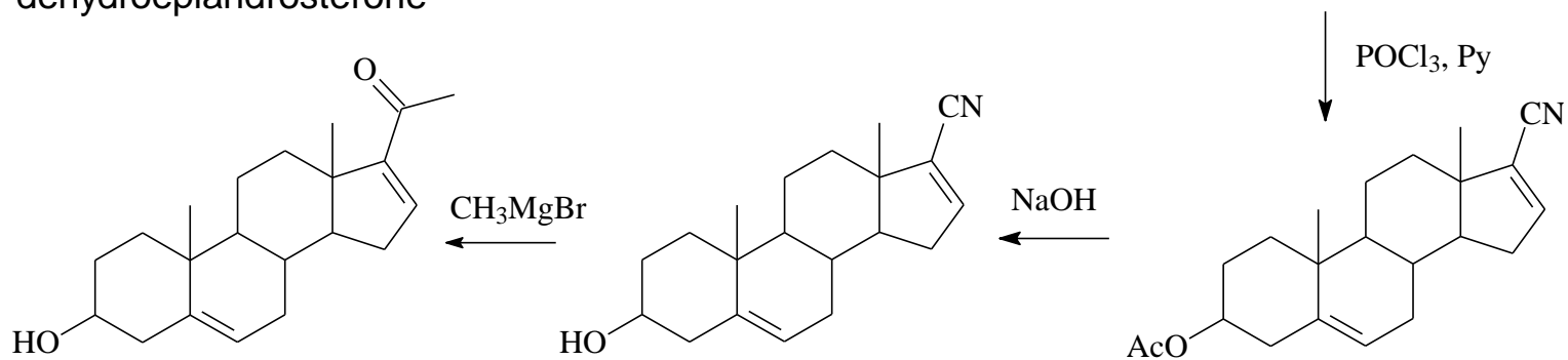
dehydroepiandrosterone
