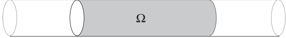
Figure 14 The surface area of \partial\Omega does not increase when the set \Omega \subset \mathbb{R}^{n-1} \times \mathbb{S}^1 is stretching.
