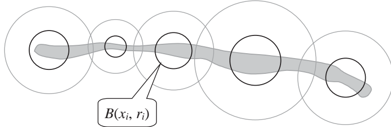
Figure 15 Set \Omega (shaded) takes in each ball B(x_i, r_i) nearly one half of its volume, whereas the balls B(x_i, 3r_i) cover all of \Omega .
