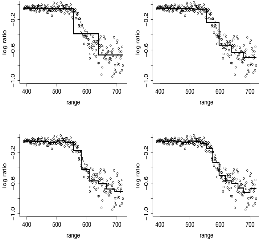
FIGURE 4.6. The LIDAR data from Example 4.5. The estimates are regressograms, obtained by averaging the Y_i s over bins. As we decrease the binwidth h , the estimator becomes less smooth.
