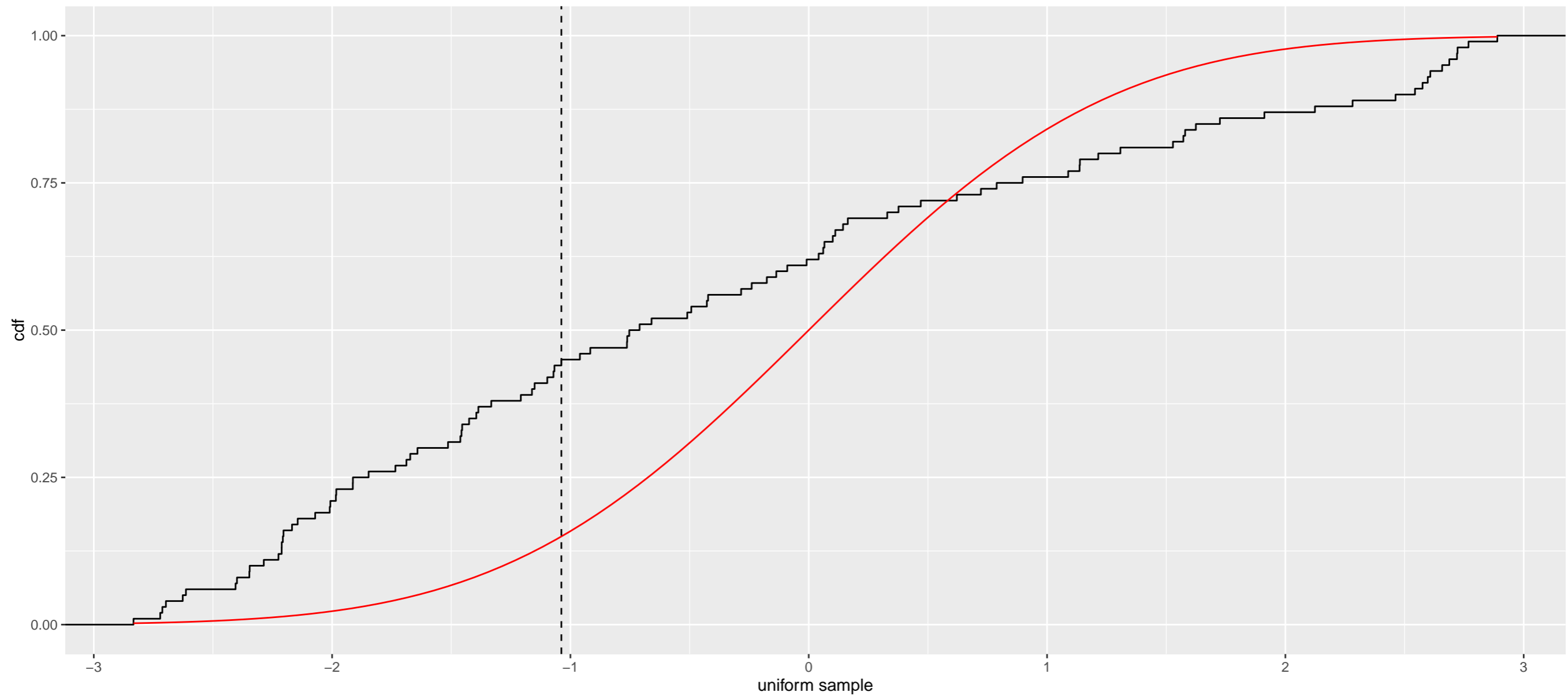
Empirical Cumulative vs Normal Cumulative Distribution Function
