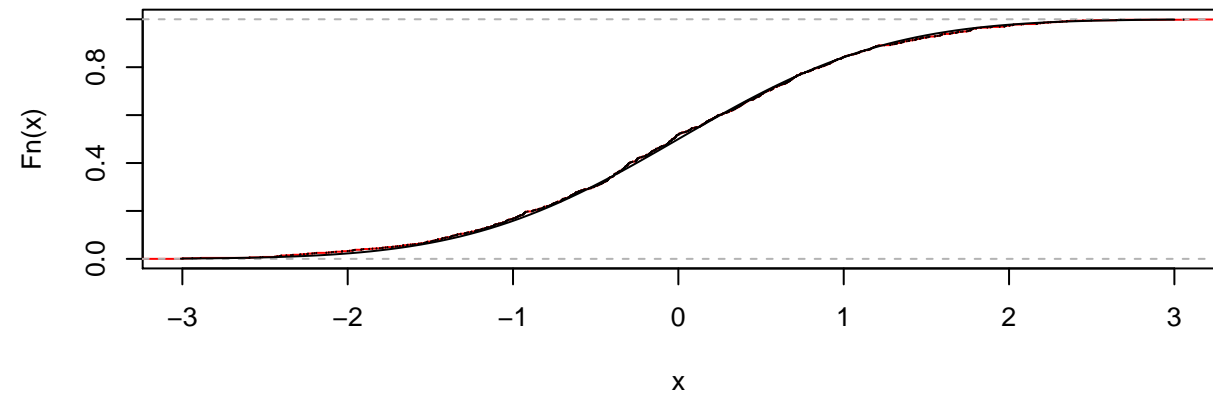
ecdf with a 1000-sample N(0,1)
