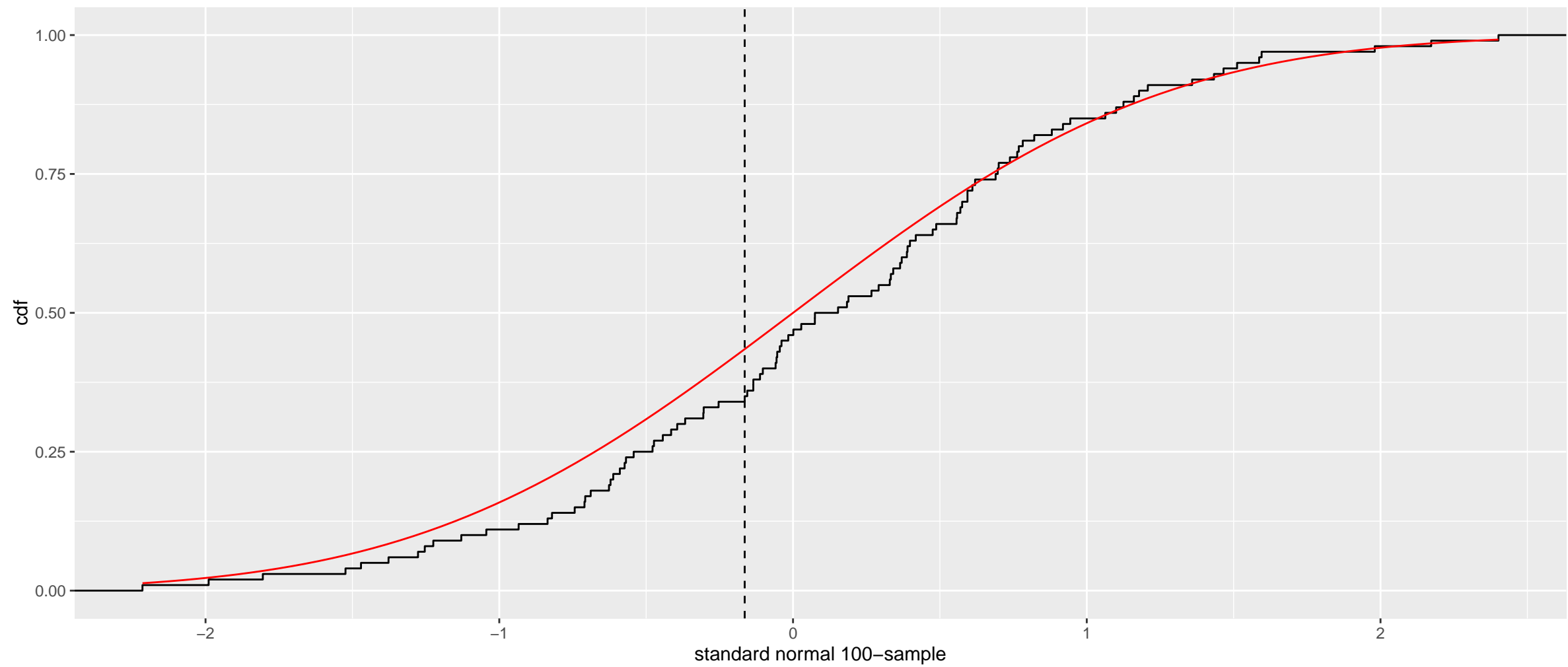
Empirical Cumulative vs Normal Cumulative Distribution Function
