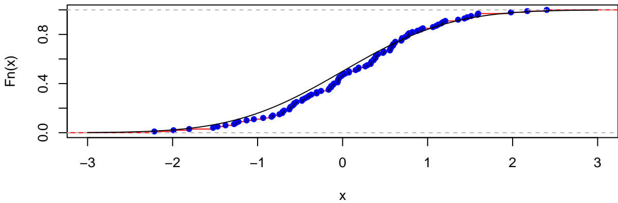
ecdf with a 100-sample N(0,1)
