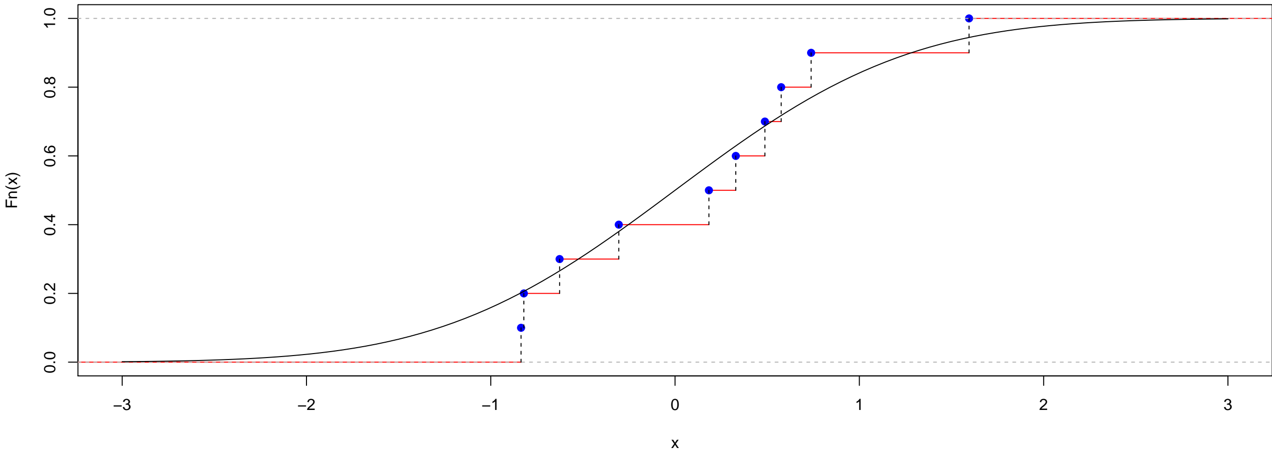
ecdf with a 10-sample N(0,1)
