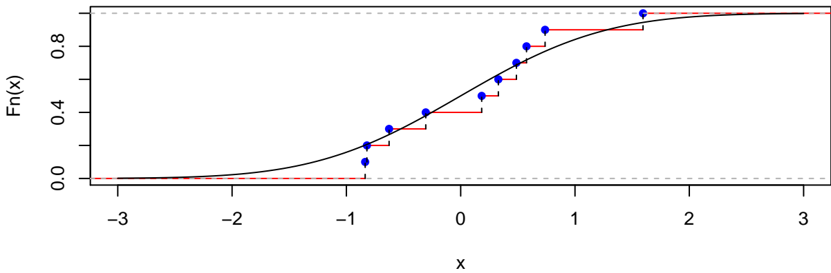
ecdf with a 10-sample N(0,1)
