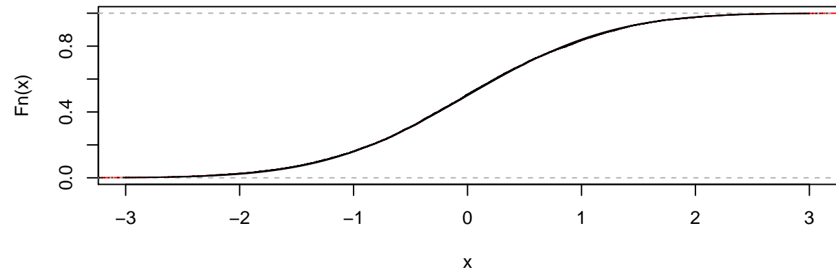
ecdf with a 10000-sample N(0,1)
