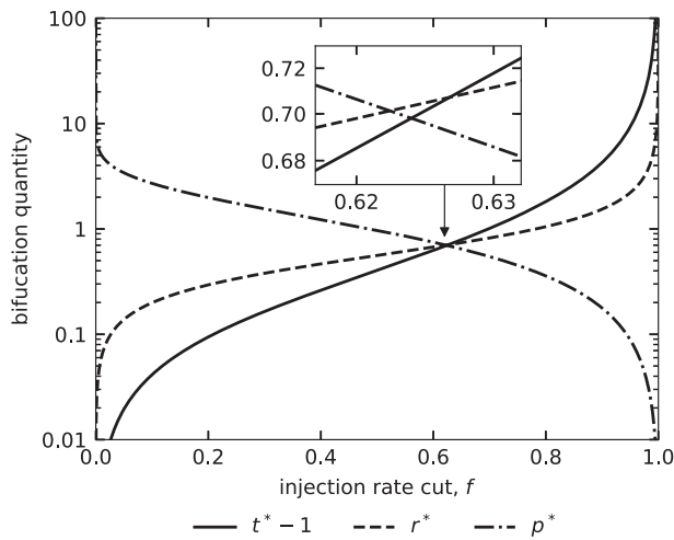
Figure 3. Variation of the bifurcation point quantities, t^* - 1 , r^* , and p^* with f . Despite appearances, the three curves do not all intersect one another at the same point, f \approx 0.62 , but rather enclose a small triangular area with vertices [ f \approx 0.6268 , t^* - 1 = r^* = 1/\sqrt{2} ], [ f \approx 0.6240 , t^* - 1 = p^* \approx 0.6981 ], and [ f \approx 0.6225 , r^* = p^* \approx 0.7012 ].
