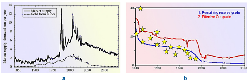
Figure 4.43 (a) the gold supply to the market as compared to gold from mining. Mining only supplies a minor part of the gold used every year by society. The amount supplied includes physical transactions also in investment, but excludes paper gold which has no substance on its own, it is a claim and not physical metal. (b) Observed and simulated ore grade. The ore grade on the Y axis is gram gold per tonne rock extracted, the X axis are the years. The red line is the GOLD model simulated, the stars represents observations on ore grades after Mudd (2007).
