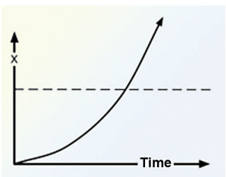
Figure 1.10 When there is unlimited growth, resource use (line) rises exponentially with time and exceeds the carrying capacity (dashes).
