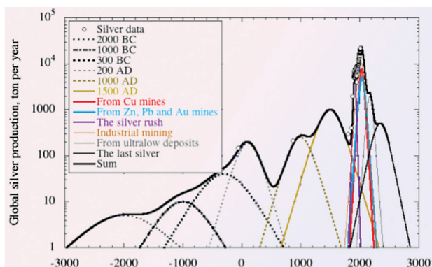
Figure 4.36 Individual and total sum of Hubbert's curves for silver production from 3000 BC to beyond 3000 AD. The parameters of the Hubbert's model used are listed in Table 4.12. The dots are observed production data.
