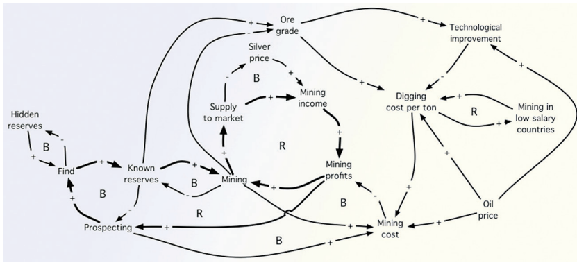
Figure 3.5 Causal loop diagram for the mining process. The mining process is mainly profit driven. The profit depends on product supply rate, supply costs and product price. For further description of the diagram see text.
