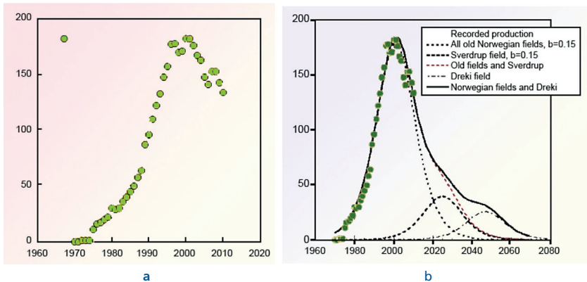
Figure 6.3 (a) Norwegian oil production to date. (b) Summary of Norwegian oil production assessment. The Sverdrup field is newly discovered in the North Sea. The Dreki field is between Iceland and Norway. Iceland has a 60% claim to the field, Norway 40%. The Dreki field is not yet fully explored and the oil quantities are therefore estimates. The Y axis in both plots are energy production millions of tonnes of oil equivalent per year.
