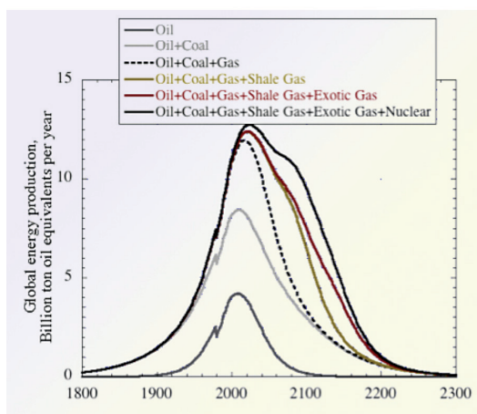
Figure 6.5 Hubbert's production curves for many different types of fossil fuels. Hubbert's curves were estimated by the authors using published reserve estimates (Al-Husseini 2009; Campbell, 2013).
