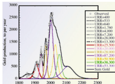
Figure 4.42 Outputs of the (a) GOLD and (b) Hubbert's models. (c) GOLD model simulation of past and future gold price in $ per troy ounce, adjusted for inflation with anchor point 2008, for the period 1950-2050. The strong ups and downs reflect different assumptions concerning derivatives and unwinding of paper gold.
