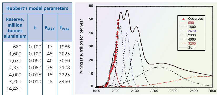
Figure 4.24 Hubbert's model assessment for aluminium extraction from bauxite.
