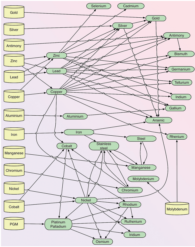
Figure 4.3 Connection between the production of many different metals and the parent metal ores. The figure shows that modelling the long-term supply of metals is a complex task, requiring computer simulation models. Cylinders stand for stocks, oval boxes for production rates.
