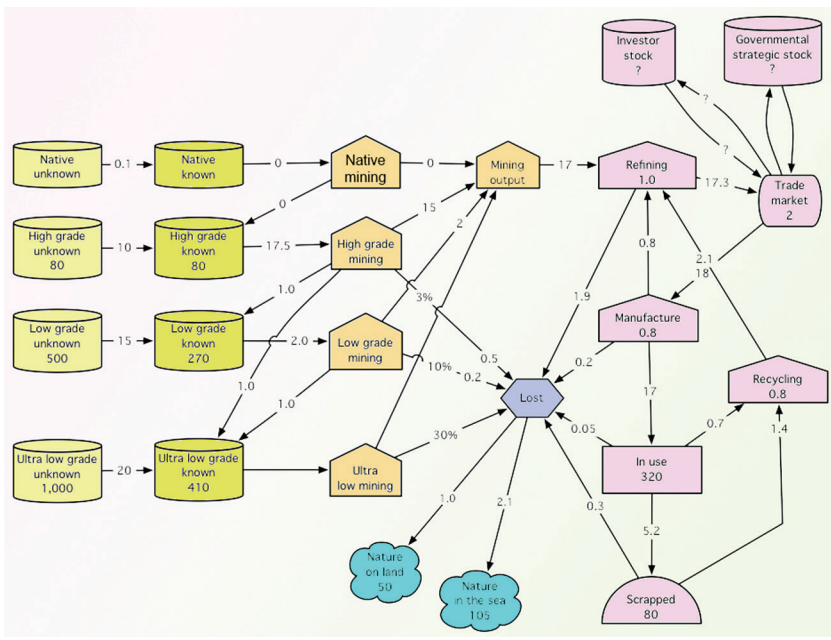
Figure 4.29 Flow chart for world copper material fluxes in 2005 in million tonnes as used in the COPPER model. Data from Gordon et al. (2006), Rauch and Graedel (2007), Radetzki (2008), Rauch and Pacyna (2009), Laherrere (2010), MinEx Consulting (2010), Crowson (2011a,b), Anglo-American Mining Corporation (2012, 2013), Kesler and Wilkinson (2013), USGS (2013).
