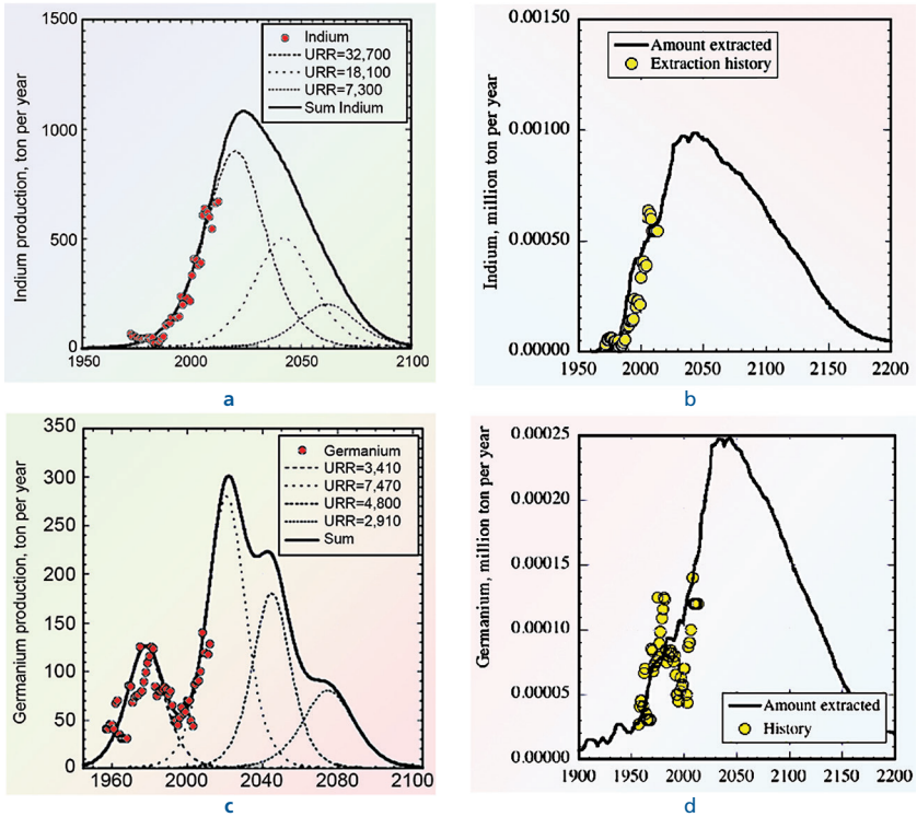
Figure 4.45 (a,b) Indium and (c,d) germanium production. Diagrams a and c are Hubbert's curves, b and d are outputs from the BRONZE model. The coloured dots are observed production data points; data are from USGS (2014). The dotted lines are sub-functions of the Hubbert's model, representing different mined deposits. Both metals are totally dependent on copper for their extraction. A systems dynamics model for these metals was used (BRONZE). X axis date in year.
