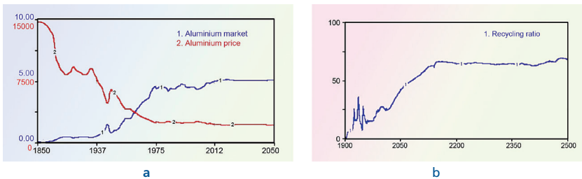
Figure 4.27 (a) Estimates of (line 1) the aluminium market stock in million metric tonne, and (line 2) the aluminium price in dollars per metric tonne. (b) The ratio of recycled material to the flux into the market. Y axis gives stock in million tonnes for the aluminium market, dollars per tonne for the price and % for the recycling rate, X axis is the year.
