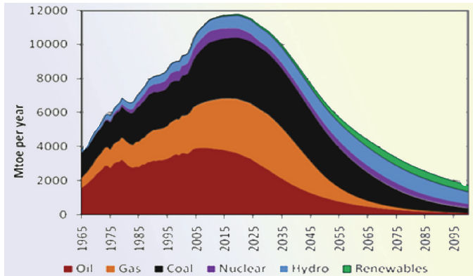
Figure 6.2 All energy in millions of tonnes per year. The figure shows that nuclear energy from uranium will not increase, that hydropower can only increase slightly and that all renewable energy can only be a fraction of fossil energy (figure published by ASPO, Association for the Study of Peak Oil in 2007; see Aleklett, 2007, and Aleklett et al. , 2012). Mtoe is million tonne oil equivalents.
