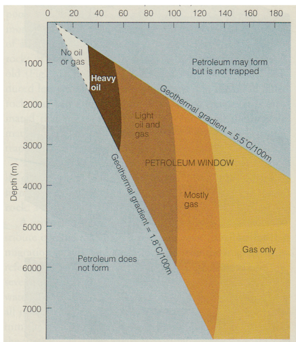
Figure 2.4 The “petroleum window” is the combination of depth and temperature within which oil and gas are generated and trapped (after Murck et al. , 1996). The X axis gives temperature in ^\circ\text{C} .
