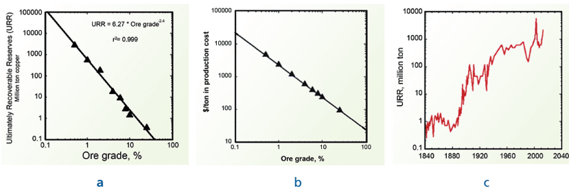
Figure 4.30 Different diagrams made to assist the assessment with the COPPER model. (a) URR as a function of the lowest ore grade assumed to be extractable. (b) Production cost per tonne versus ore grade. (c) URR as a function of time for copper. As we go down in ore grade, it theoretically may look as if the reserve increases fast, but at the same time, the decreasing yield makes this irrelevant as we cannot extract it efficiently.
