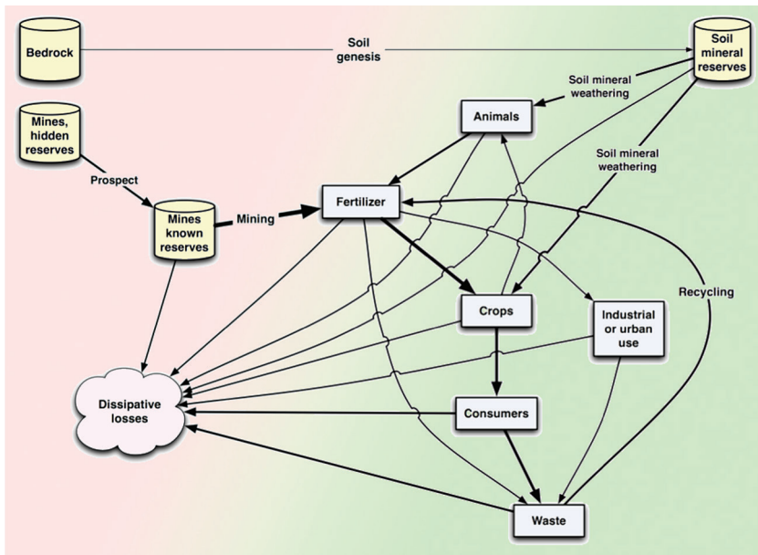
Figure 5.4 Flow chart of the phosphorus cycle. Flow charts are used together with the causal loop diagrams to define the simulation model used here (after Sverdrup and Ragnarsdottir, 2011).
