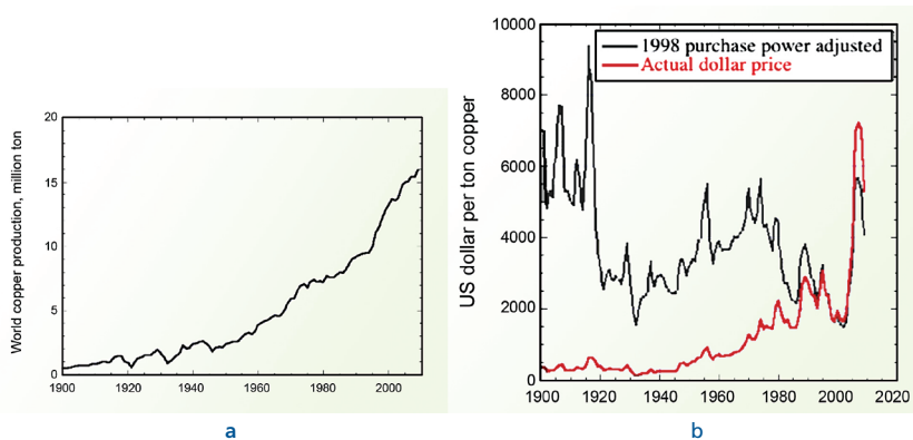
Figure 4.28 (a) The global copper production from mines, 1900–2010. Data adapted from the USGS (2012) database. (b) Running and value-adjusted copper market price 1900–2010.
