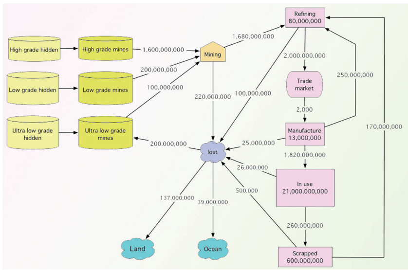
Figure 4.12 Flow chart for iron 2010. Amounts in million tonnes of iron. In society, the stock is estimated to be about 21 billion tonnes (after Rauch and Pacyna, 2009).
