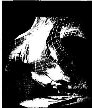
CADCAM system
