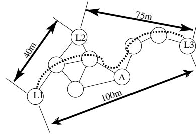
Fig. 2. “DV-hop” correction example
