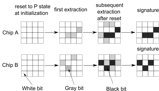
FIGURE 8. Operation sequence for extracting a PUF signature from a 4 \times 4 STT-MRAM array. The extracted data is categorized into three patterns: much less than 50% (white), around 50% (gray) and much more than 50% (black). After [20].
