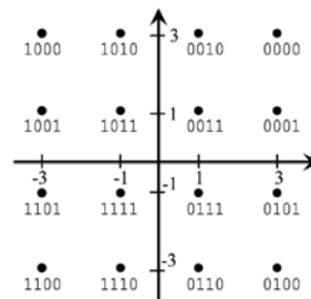
16-QAM (4 bits/symbol)
