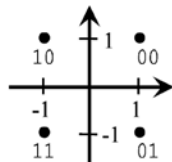
QPSK (2 bits/symbol)
