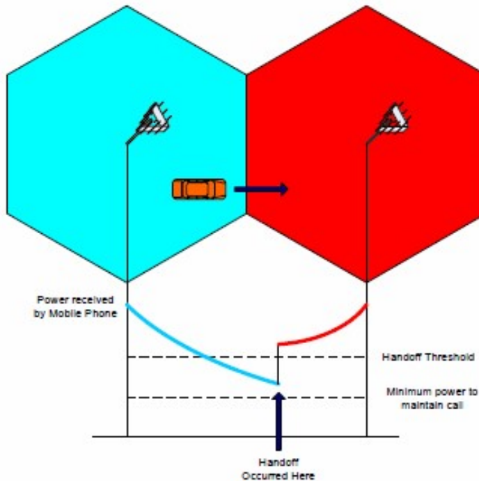
Successful Handoff
