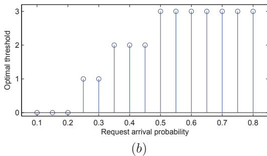
Fig. 3. (a) Hit rate under different thresholds and (b) optimal threshold.
