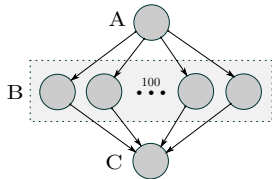
Figure 1: A split (A), compute(B), and merge(C) dataflow.
