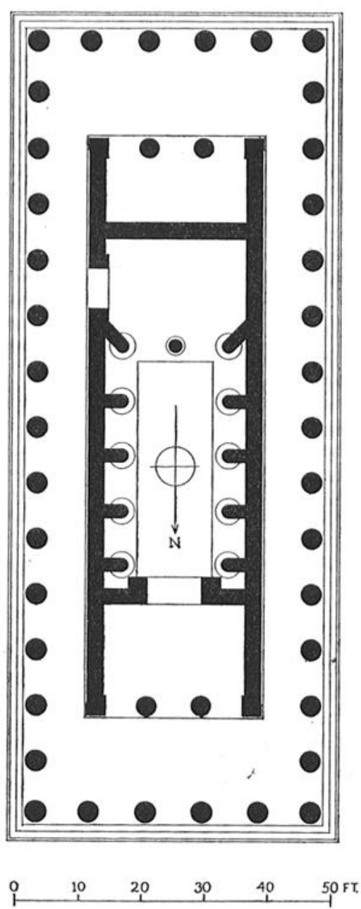
FIG. 56.—TEMPLE OF APOLLO EPICURIUS AT BASSAE.
