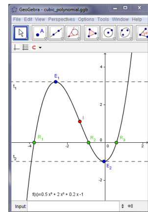
GeoGebra window after the size reduction
