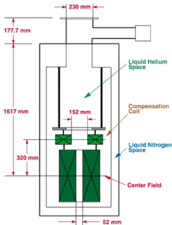
20T Superconducting Magnet
