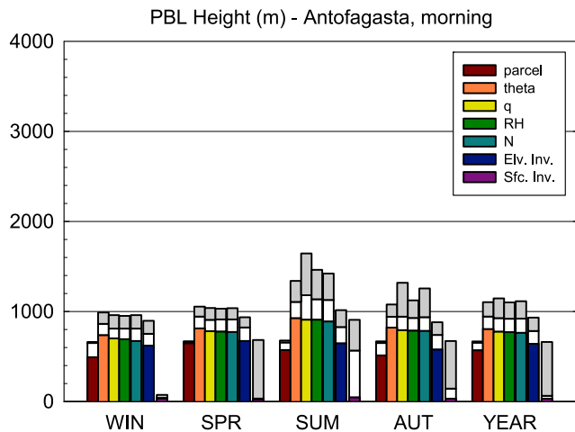
Figure 7. Same as Figure 5 but for Antofagasta, Chile ( 22^{\circ}\text{S} , 137^{\circ}\text{W} ), for morning only.
