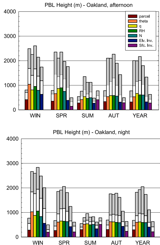
Figure 6. Same as Figure 5 but for Oakland, California ( 38^{\circ}\text{N} , 122^{\circ}\text{W} ), for afternoon and nighttime.
