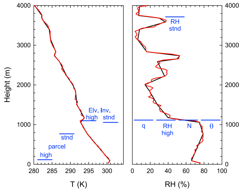
Figure 9. Effect of sounding vertical resolution on estimated PBL heights (m) at Koror Island, Republic of Palau (7°N, 134°E), for the 1200 UTC sounding of 21 February 2007. Standard-resolution and high-resolution (black and red curves, respectively) (left) temperature (K) and (right) relative humidity (%) soundings are shown, along with the PBL heights identified by six methods. For the parcel, elevated inversion, and RH gradient methods, estimated heights differ for the high-resolution and standard-resolution cases. For the q , N , and \Theta gradient methods, estimated PBL heights are the same.
