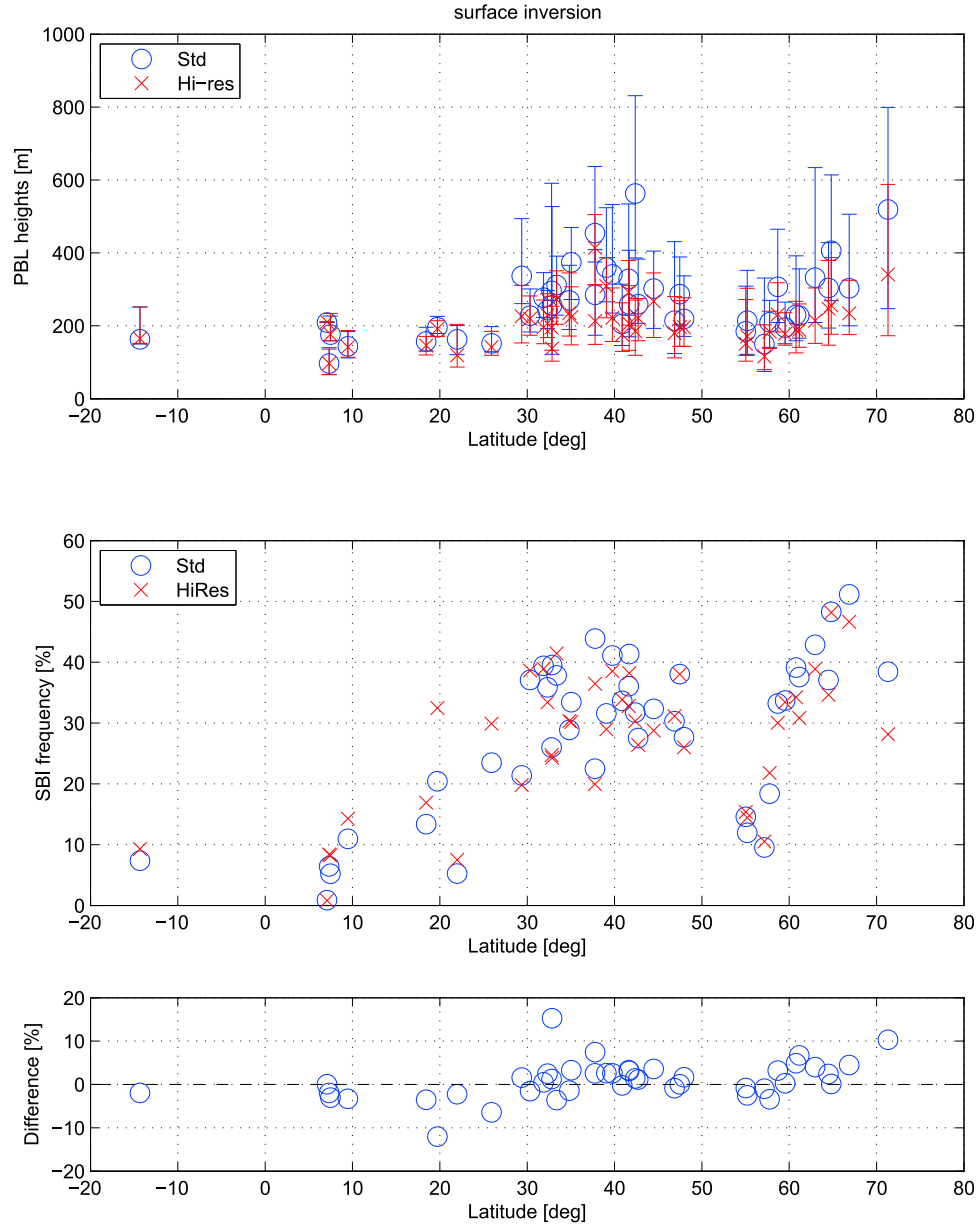
Figure 11. (top) Same as Figure 10, but showing results for the height of the top of surface-based inversions (SBI). (middle) Frequency (%) of SBI occurrence based on standard (blue) and high vertical resolution (red) data. (bottom) Difference (standard minus high resolution) in SBI frequency.
