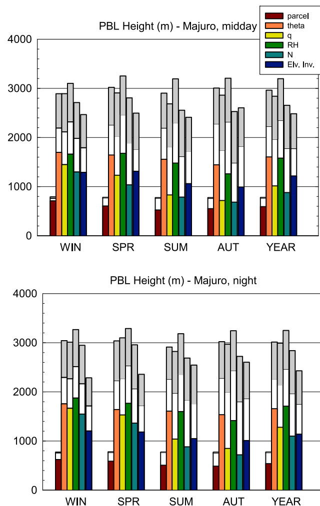
Figure 8. Same as Figure 5 but for Majuro Atoll, Marshall Islands ( 7^{\circ}\text{N} , 171^{\circ}\text{E} ), at midday and nighttime.
