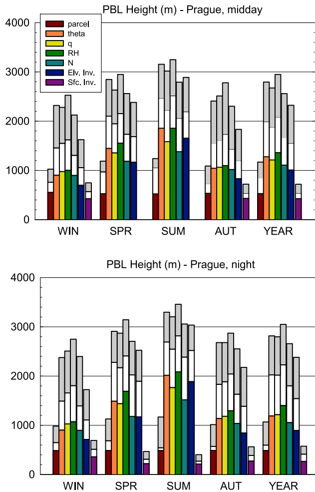
Figure 5. Seasonal and annual quartile values of planetary boundary layer height (m above ground level) at Prague, Czech Republic ( 50^{\circ}\text{N} , 14^{\circ}\text{E} ), based on data for 1999–2008. For each method, the 25th, 50th, and 75th percentile values are shown (in colored, white, and gray bars, respectively), for (top) midday and (bottom) nighttime. Heights based on surface-based inversions are from a different set of soundings than heights based on the other methods. They are not shown for daytime for some seasons at Prague because they occur rarely (1% of soundings).
