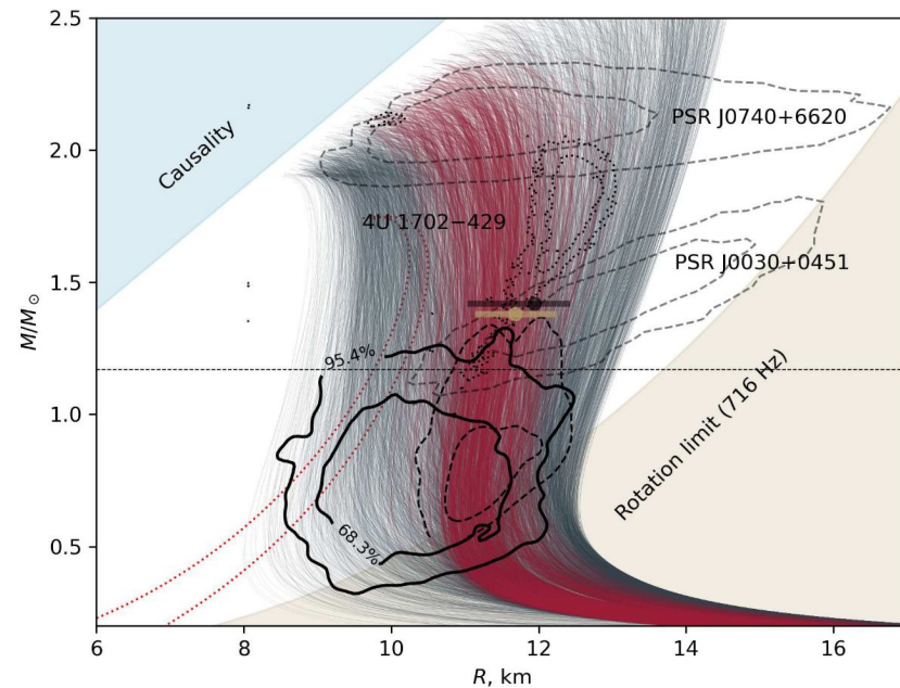
A strangely light neutron star
