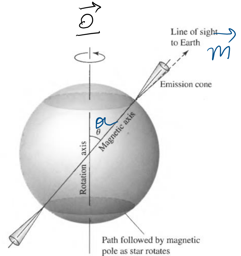
FIGURE 16.25 A basic pulsar model.
