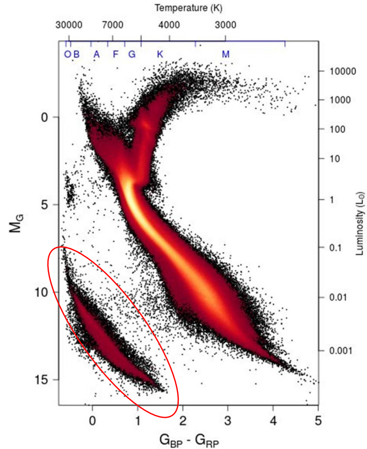
Gaia DR3 HR Diagram of low extinction and accurate parallax sources (in the Galaxy)
