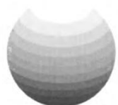
\ell = 1, m = 0
