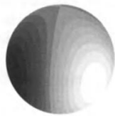
\ell = 2, m = \pm 2
