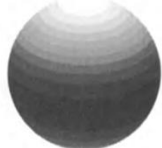
\ell = 2, m = 0
