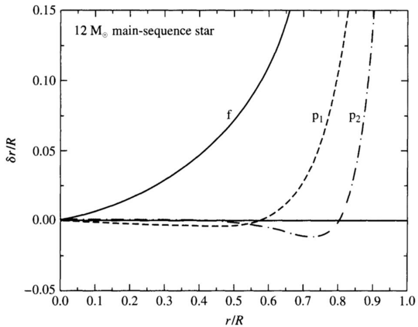
Nonradial p-modes with l = 2
