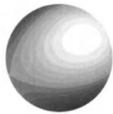
\ell = 2, m = \pm 1
