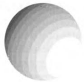
\ell = 1, m = \pm 1
