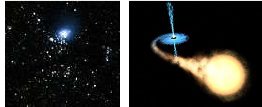
M33 X-7 X-ray binary 15.7 M_{\odot} black hole.
