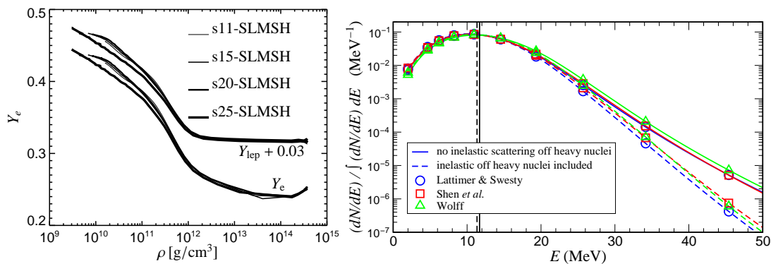
Figure 4. Left: The evolution of the electron-to-baryon ratio Y_e and the lepton-to-baryon ratio Y_{lep} as function of central density for stars with masses between 11 and 25 M_\odot . (from [7]). Right: Comparison of the normalized neutrino spectra, arising from the \nu_e burst shortly after bounce, without (solid) and with (dashed) consideration of inelastic neutrino-nucleus scattering in the supernova simulations and for 3 different Equations of State. (from [30]).
