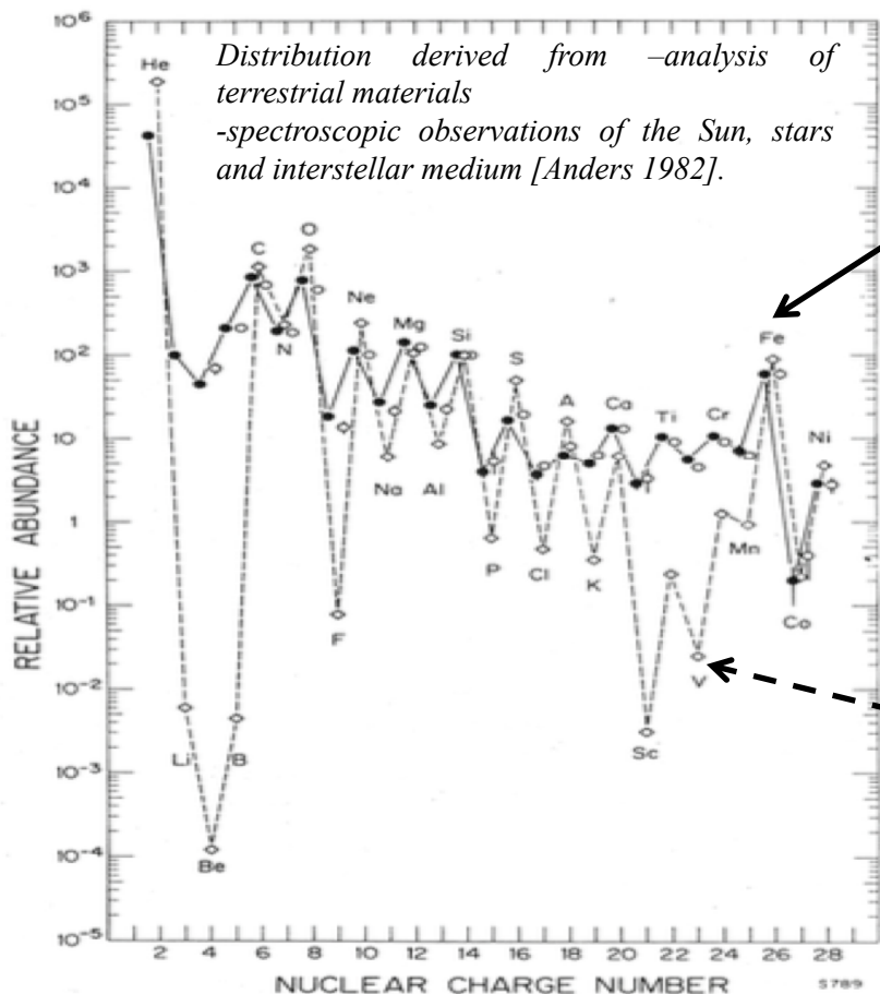
Fig. 11. Elemental abundances of cosmic rays from helium to nickel measured at Earth, compared to the solar system (or universal) abundance scale, all relative to silicon. Solid circles: low energy ( 70-280 \text{ MeV amu}^{-1} ); open circles: high energies ( 1000-2000 \text{ MeV amu}^{-1} ); open diamonds: solar system abundances (figure from [Simpson 1983]).
