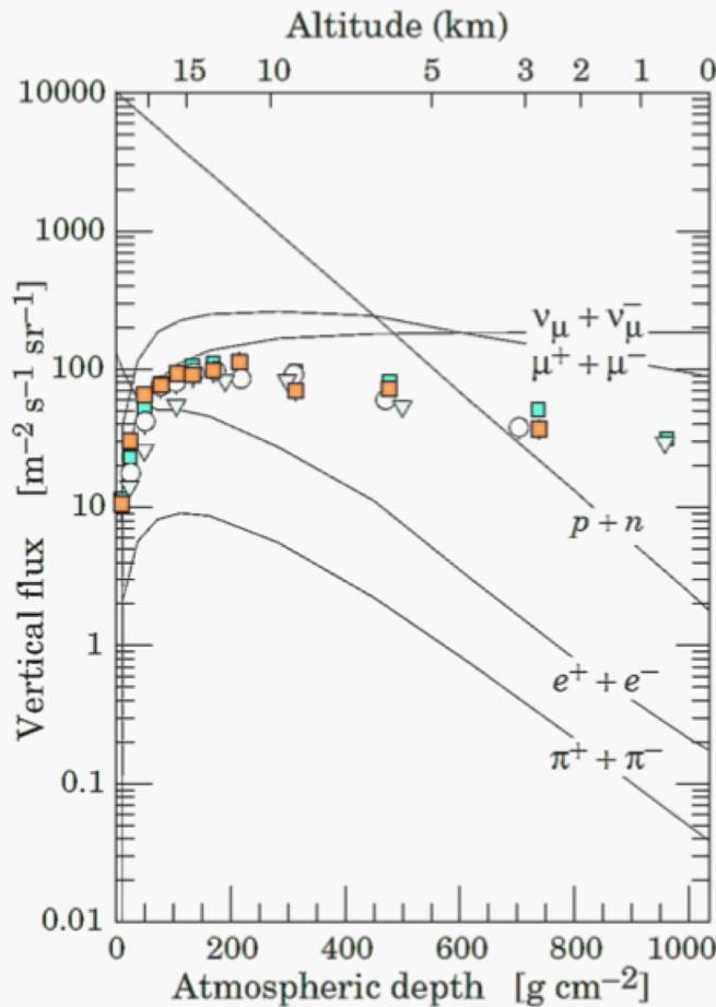
Figure 29.4: Vertical fluxes of cosmic rays in the atmosphere with E > 1 GeV. The points show measurements of negative muons with E_\mu > 1 GeV [41–45].
