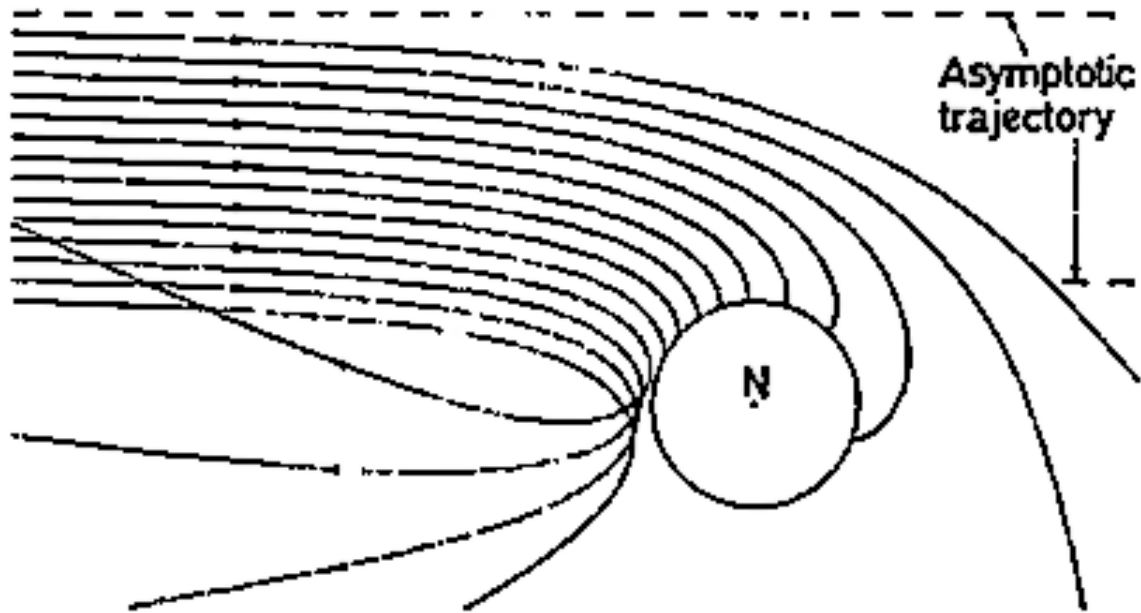
Trajectories of 20 GeV positively charged particles in the equatorial plane.
