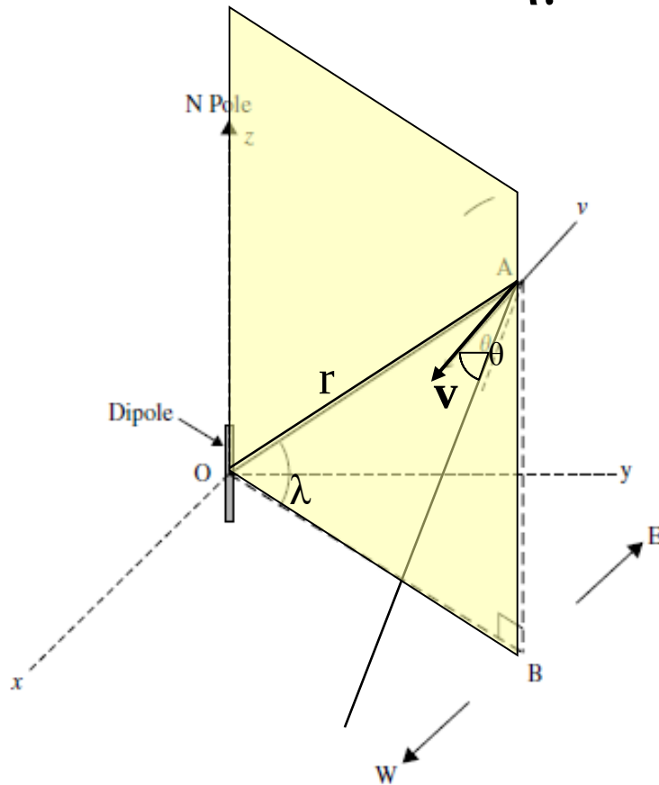
Fig. 9.4 Coordinate system and variables describing a particle A with velocity \mathbf{v} in the field of a dipole M at O. \theta is the angle between the velocity vector \mathbf{v} of the particle and the meridian plane OAB rotating with the particle.
