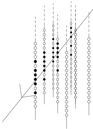
Fig. 10.23. Sketch of the detection technique with a deep underwater neutrino telescope. Upward-going neutrino-induced muon goes through the detector and generates Cherenkov light in a wide cone. The track is reconstructed from the timing of the triggered photomultipliers, shown here with full circles.
