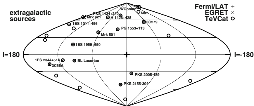
Fig. 10.9. Twenty-three TeV \gamma -ray sources listed in TeVCat are shown with circles in galactic coordinates. The sources detected by EGRET are marked with 'x's and those from the Fermi/LAT list of bright \gamma -ray sources are marked by pluses.
