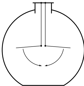
Fig. 5.1. Schematic drawing of an electroscope such as that used by Hess in the discovery of cosmic rays.
