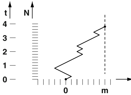
Fig. 4.5. One-dimensional diffusion problem. The particle scatters either left or right at every time step.
