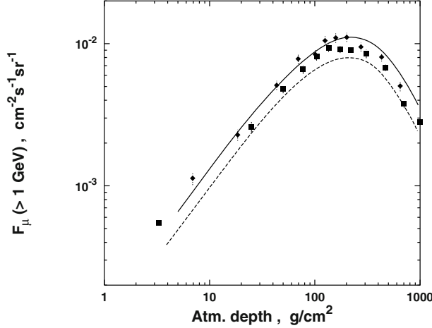
Fig. 6.8. Muon growth curve. The full squares are from Ref. [172] and the diamonds are from Ref. [176]. The predictions are from Refs. [165, 174], shown with a full and a dashed line respectively.
