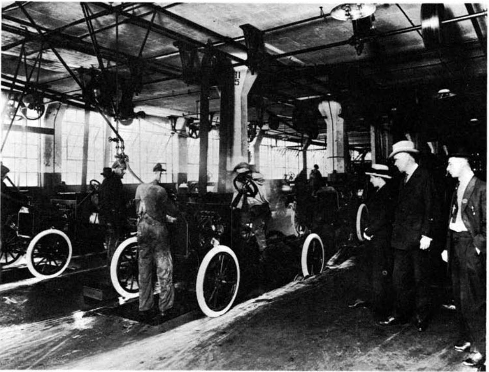
FIGURE 6.31. Driving Off the Assembly Line, Highland Park, 1914. At the end of the line, workmen filled the radiator and started the engine before driving off the line. (Henry Ford Museum, The Edison Institute. Neg. No. 833-997.)
