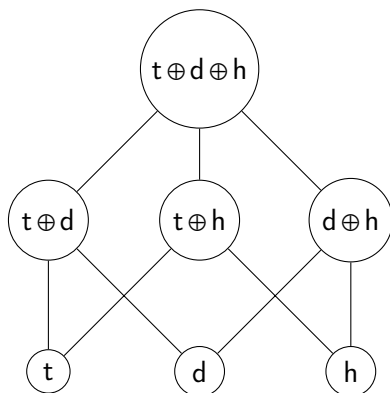
Figure 10.1: An algebraic structure
