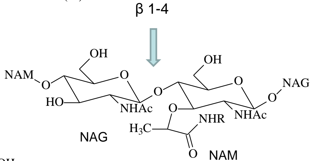
muramic acid (M)
