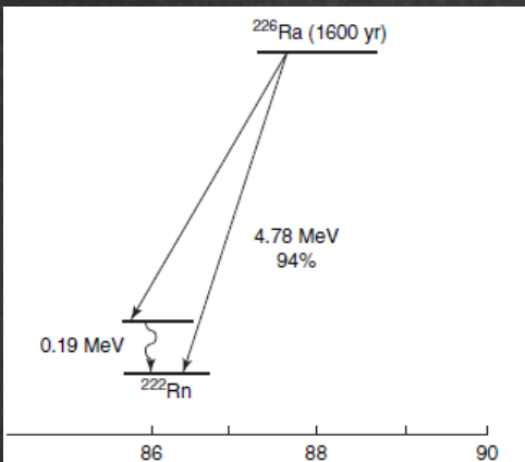
Figure 1.11 Radioactive decay scheme for \alpha decay of ^{226}\text{Ra} .
