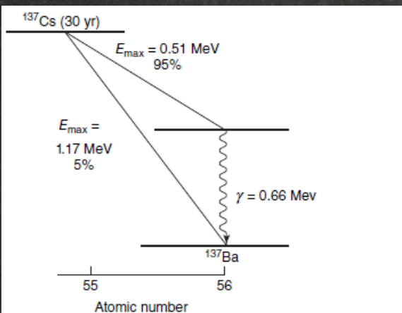
Figure 1.12 Radioactive decay scheme for electron decay of ^{137}\text{Cs} .
