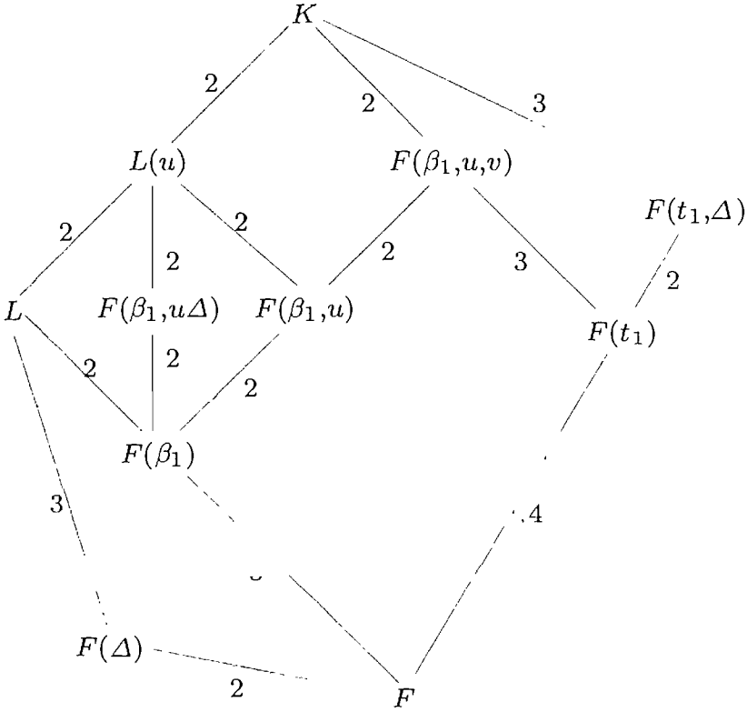
FIGURE 13.1. Field tower for F(t_1, t_2, t_3, t_4)/F .
