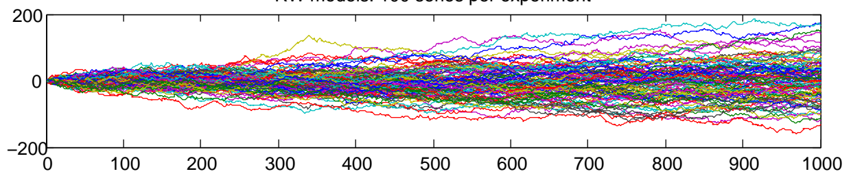
RW models: 100 series per experiment
