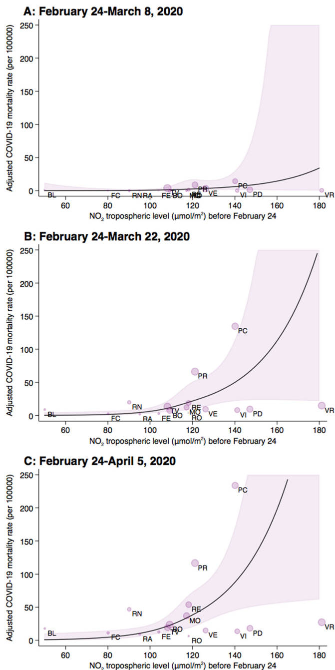
Fig. 2. Negative binomial regression analysis between nitrogen dioxide ( \text{NO}_2 ) tropospheric levels ( \mu\text{mol}/\text{m}^2 ) before the spread of the outbreak and COVID-19 mortality rate (deaths per 100,000) in the three periods after the lockdown dates (A: February 24–March 8; B: February 24–March 22; C: February 24–April 5). Adjusted COVID-19 mortality rate (solid line) with 95% confidence interval (dash lines) was estimated with a multivariable model, taking into account population density, aging index, people mobility measured from telephone movements before the lockdown, temperature ( ^{\circ}\text{C} ) and relative humidity (%) in the three subsequent periods, and airport presence. Shaded circles are weighted on number of deaths corresponding to the adjusted mortality rates at each time point.
