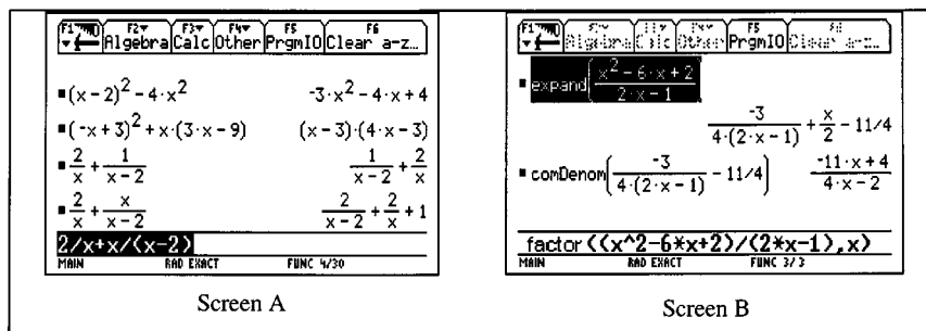
Figure 3. Algebraic tasks.
