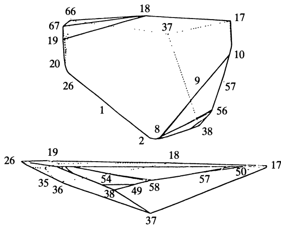
Two views of a 38-faced polytope with 70 vertices, discovered by Engel (1980)
