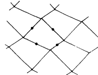
for triangles use symmetries
