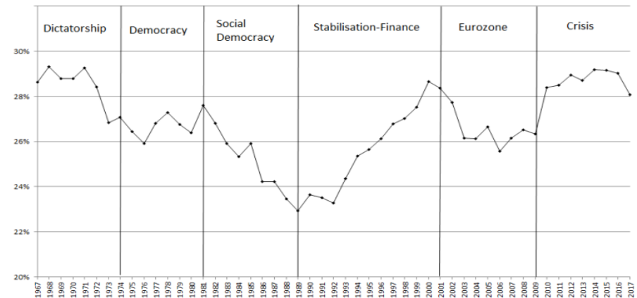
Figure 1: The top decile
