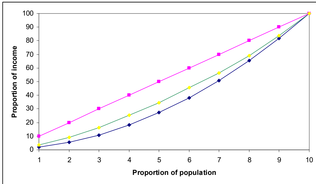
Figure 1. Lorenz curves
