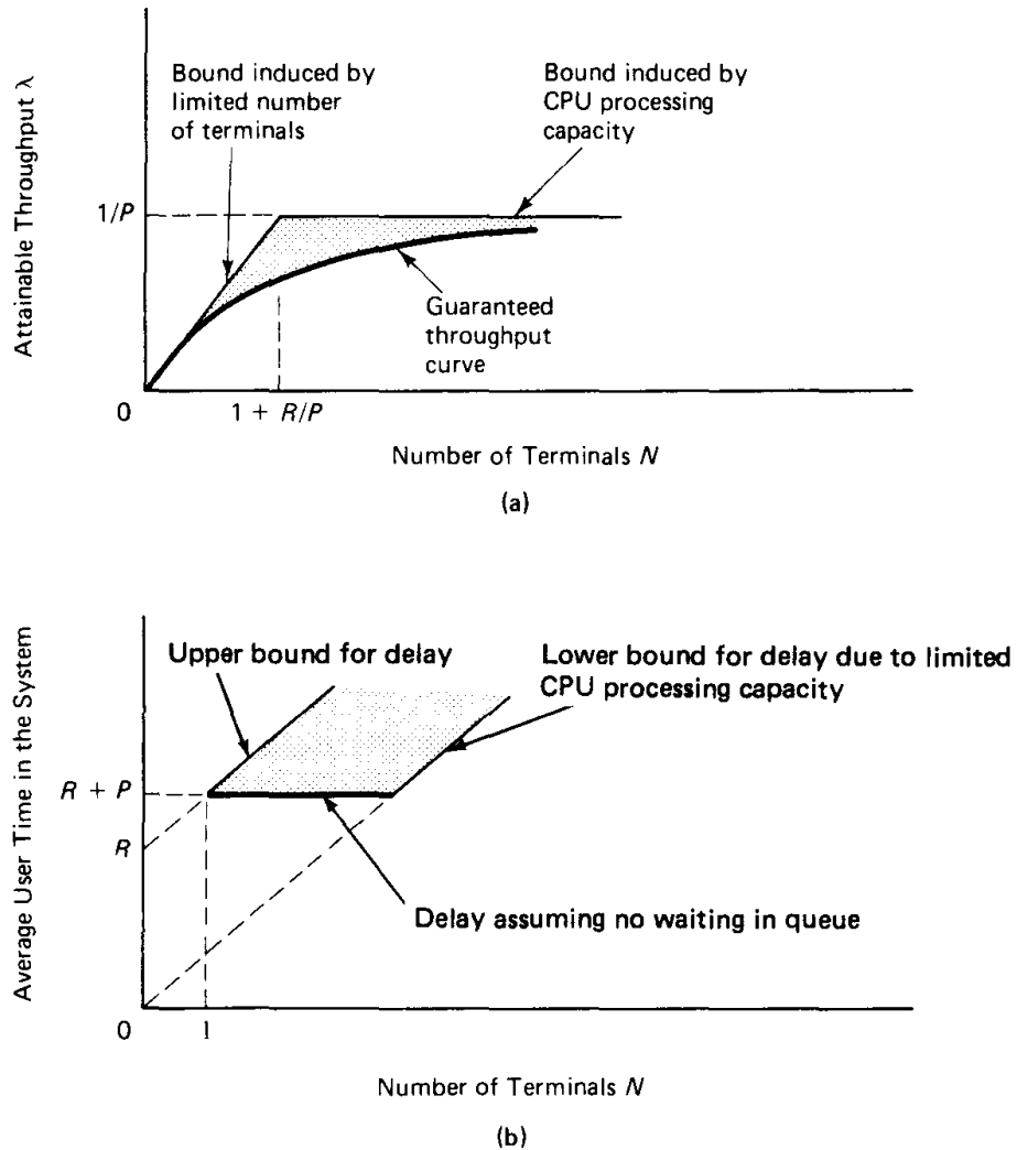
Figure 3.5 Bounds on throughput and average user delay in a time-sharing system. (a) Bounds on attainable throughput [Eq. (3.8)]. (b) Bounds on average user time in a fully loaded system [Eq. (3.9)]. The time increases essentially in proportion with the number of terminals N .
