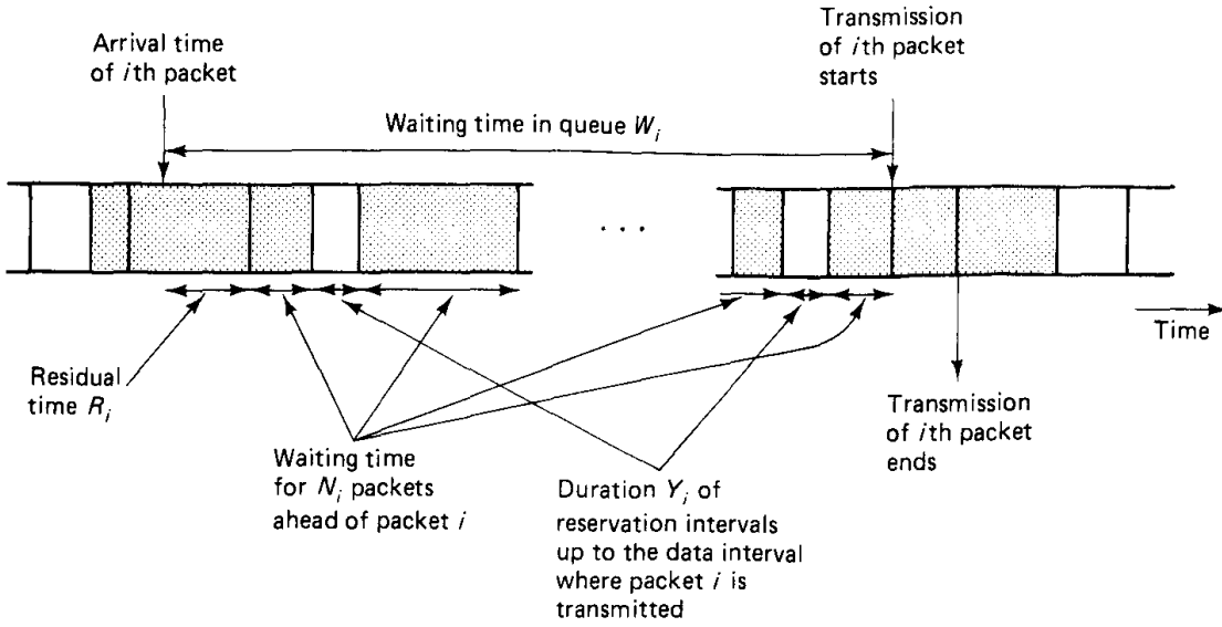
Figure 3.23 Calculation of the average waiting time in the multiuser system. The expected waiting time E\{W_i\} of the i^{\text{th}} packet is
