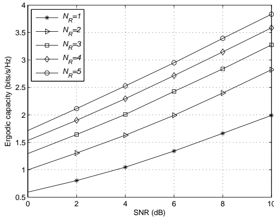
Figure 3. Ergodic capacity for MIMO systems
