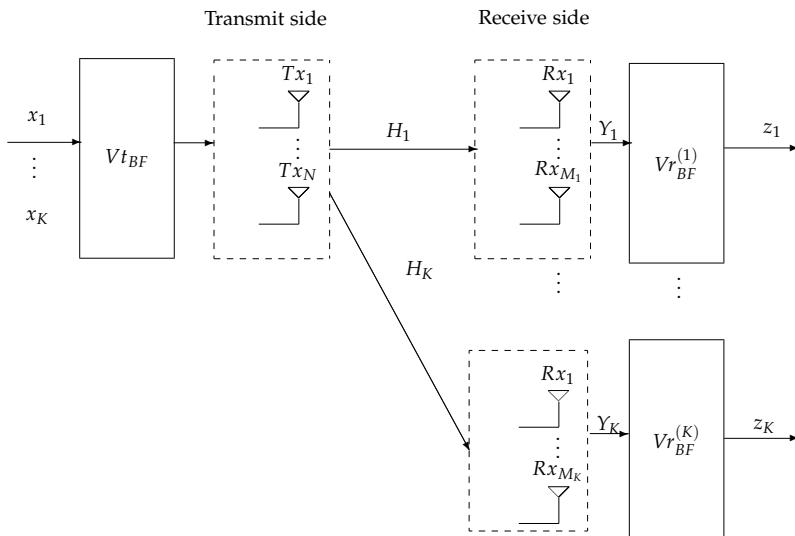
Figure 12. MU-MIMO with beamforming
