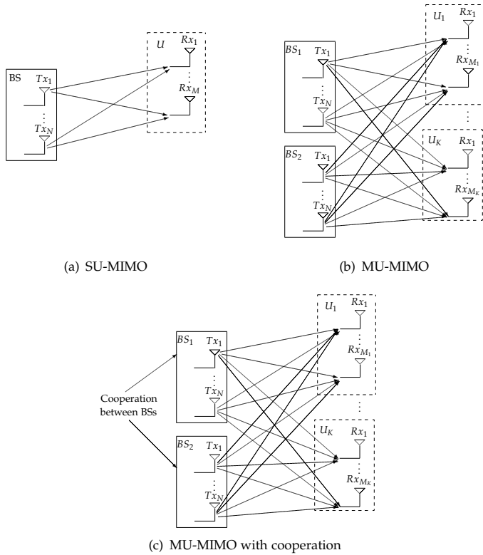
Figure 5. MU-MIMO configurations
