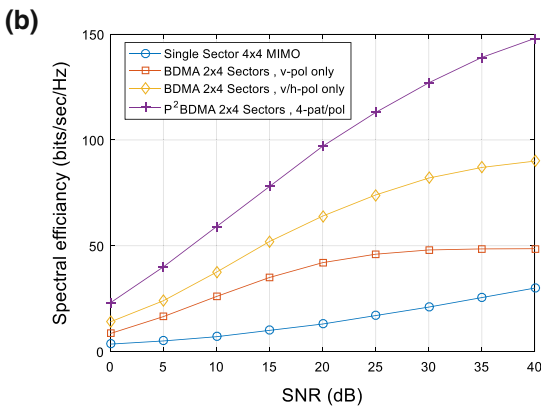
Fig. 6 a Pattern/polarization antenna elements for massive MIMO b Downlink spectral efficiency vs. SNR
