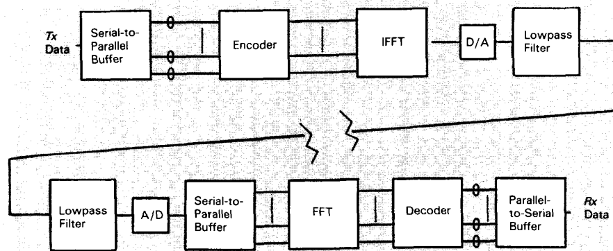
Fig. 7. Basic multicarrier "mo-dem."
