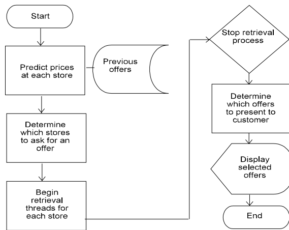
Figure 1. Flow-diagram illustrating the operational decision process for a shopbot.
