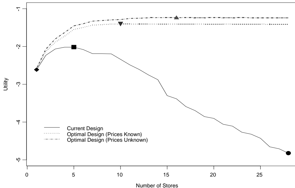
Figure 3 Expected utility based upon the number of stores that are queried using several different shopbot designs.
