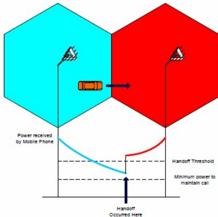
Successful Handoff
