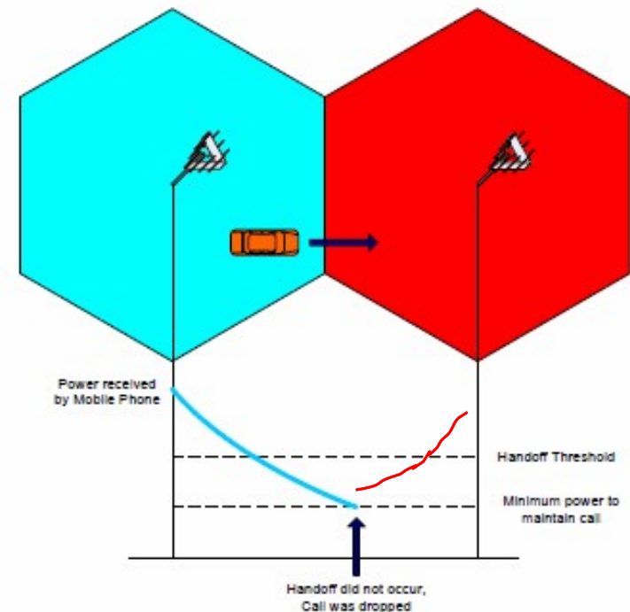
Unsuccessful Handoff
