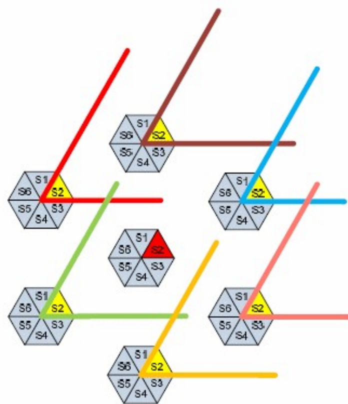
60 degrees Sectoring
