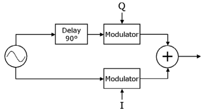
Figure 9-2. Quadrature Modulation.
