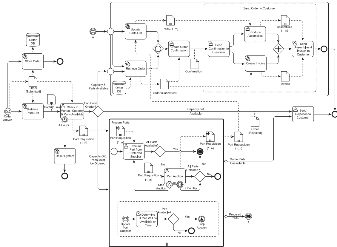
FIGURE 8 An example of a standalone Process (Orchestration) diagram.
