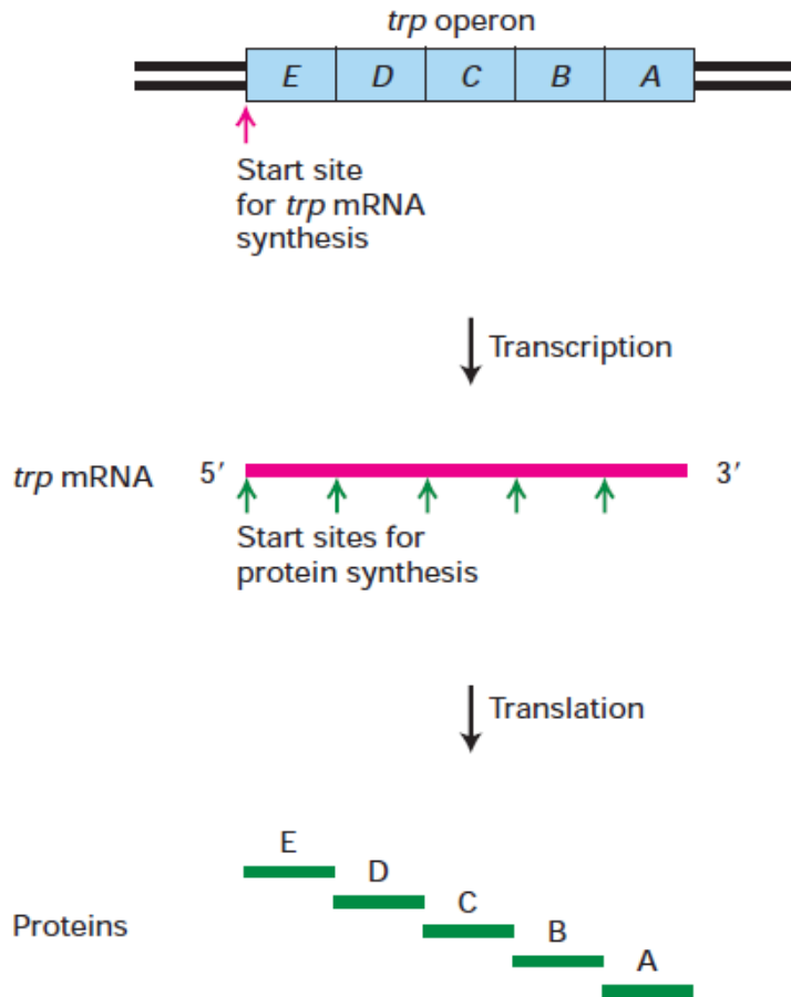
(a) Prokaryotes
