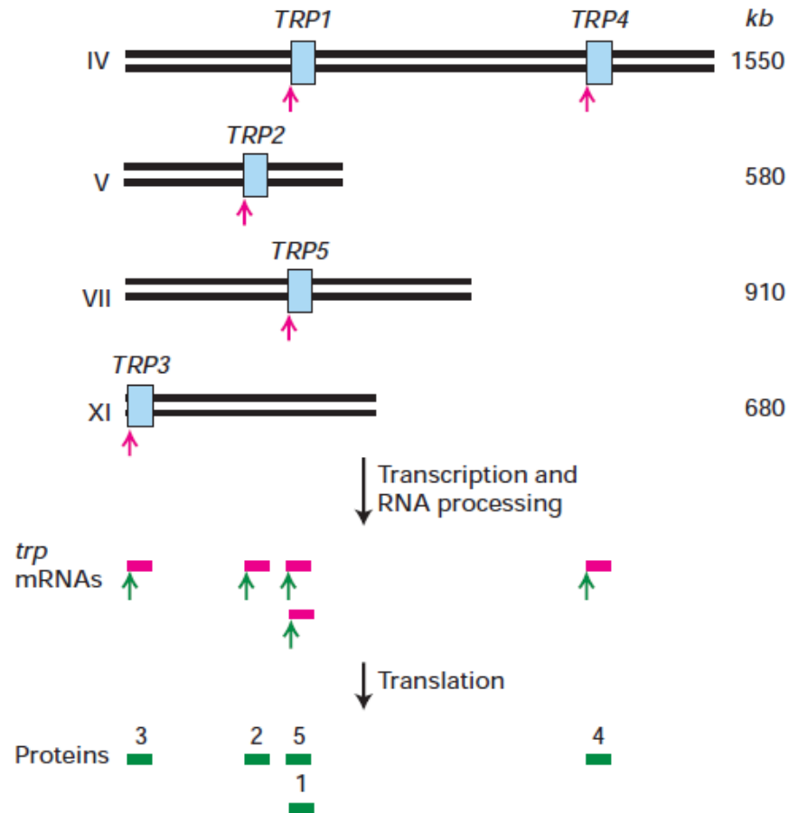
(b) Eukaryotes
