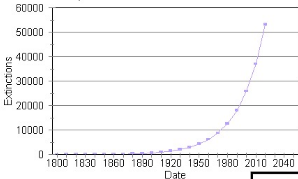
Species Extinctions Since 1800
